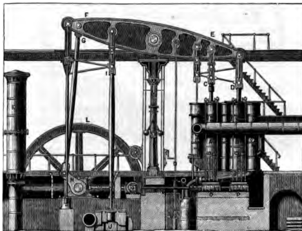
FIG. 105.—Double-Cylinder Pumping-Engine, 1878.
